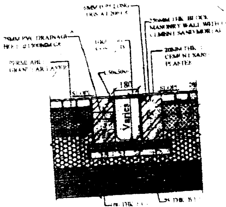
300 WIDE DRAIN CROSS SECTION (SCALE: 1/20)
